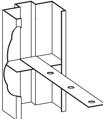
T-Anchor
